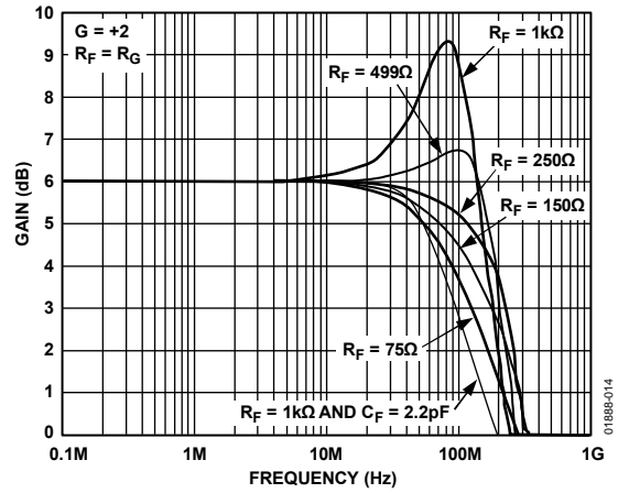
Figure 14. Small Signal Frequency Response vs. Frequency and R_F , Noninverting, V_{OUT} = 50 \text{ mV p-p} (See Figure 48)
