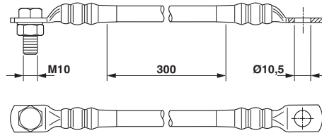
Dimensional drawing
