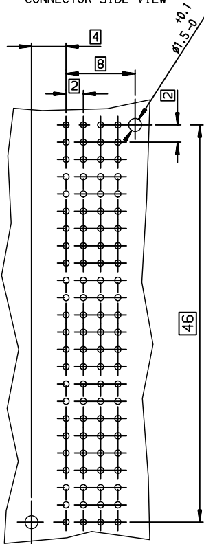
LAYOUT FOR P.C.B CONNECTOR SIDE VIEW
