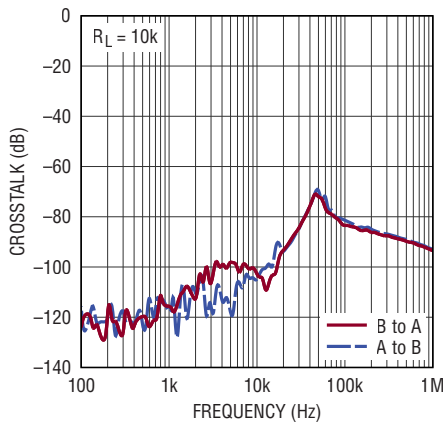
LTC2067 Crosstalk vs Frequency
