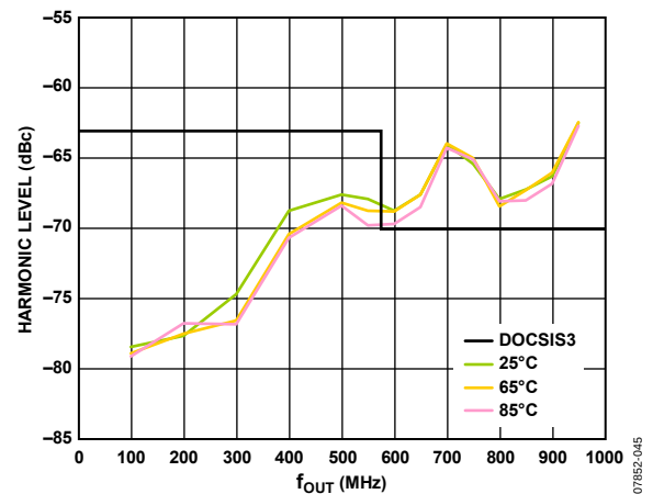
Figure 30. Second Harmonic Performance vs. f_{OUT} over Temperature, 2-Channel QAM, f_{DAC} = 2.3 GHz, Full-Scale Current = 25 mA, Sum Scale = 32 (DOCSIS SPEC Is -70 dBc; Harmonic Exception Is -63 dBc)
