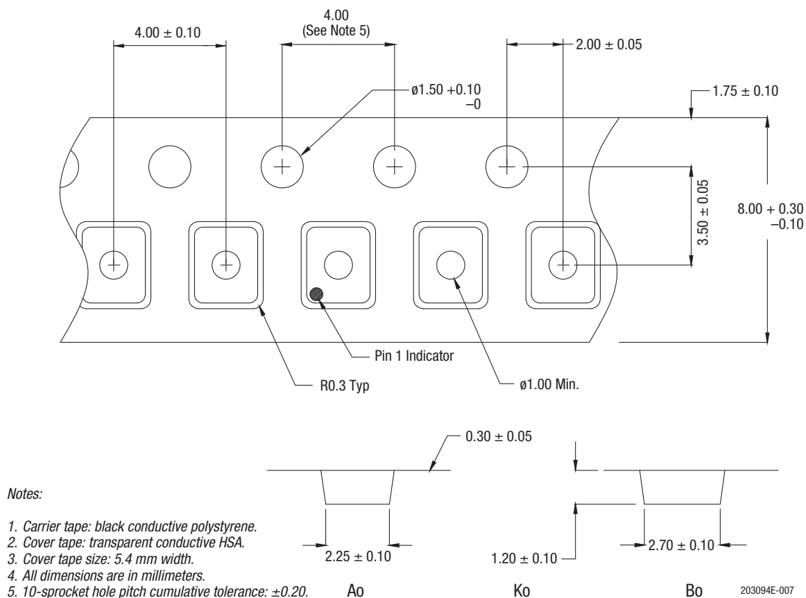
Figure 8. SKY65450-92LF Tape and Reel Dimensions
