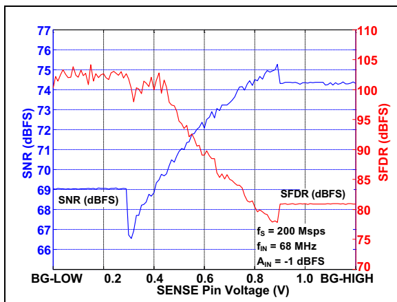
FIGURE 3-19: SNR/SFDR vs. SENSE Pin Voltage: f_s = 200 Mpsps, f_{IN} = 68 MHz.
