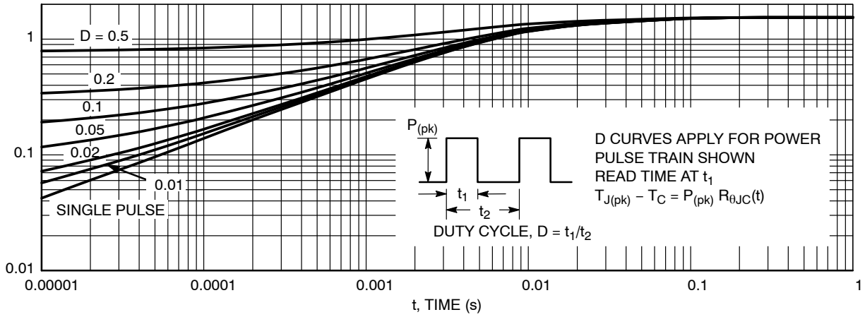
Figure 12. Thermal Response
