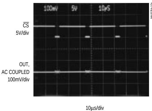
MAJOR-CARRY TRANSITION
