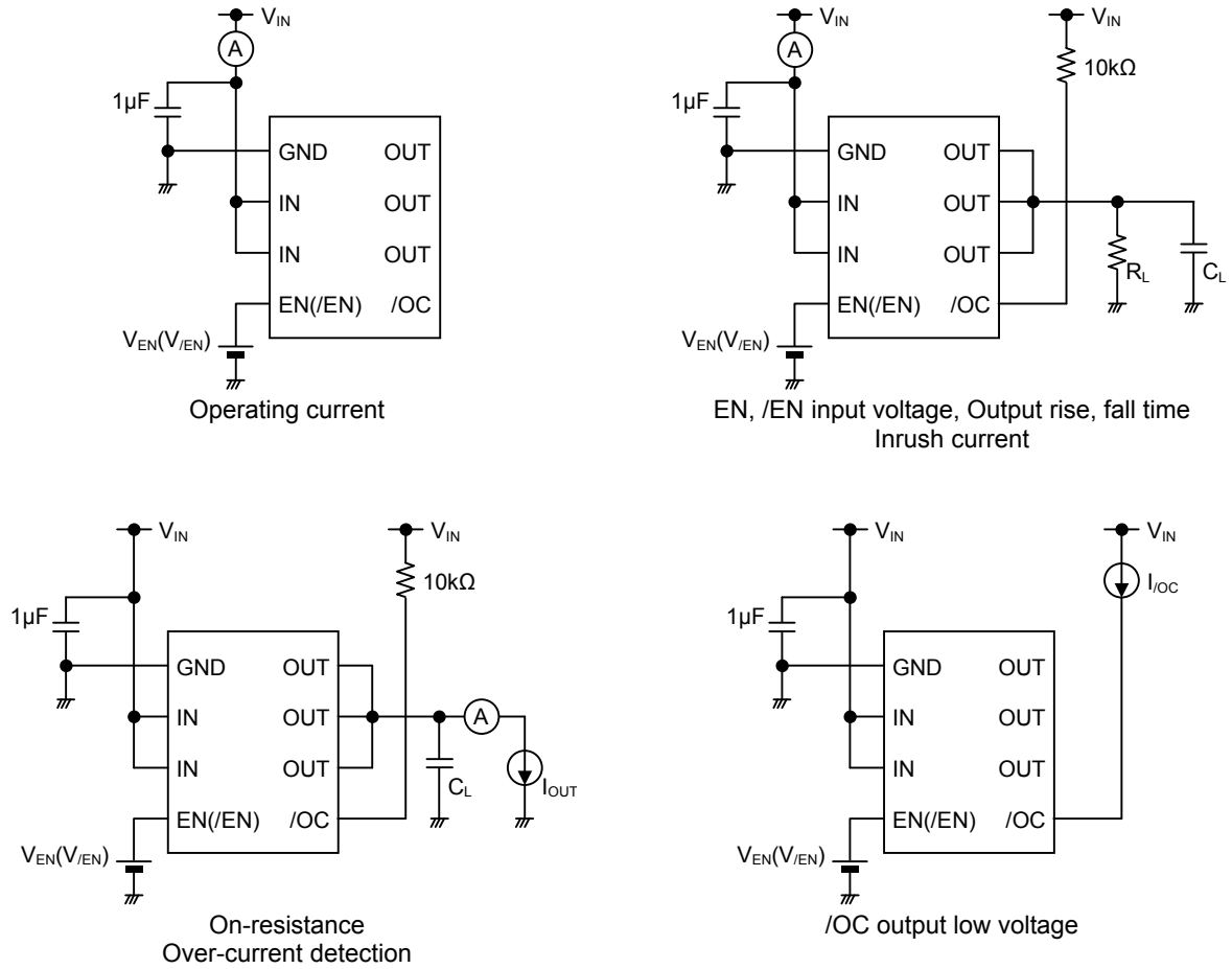
Fig.1 Measurement circuit
