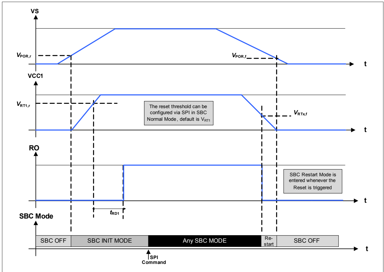
Figure 57 Ramp up / down example of Supply Voltage
