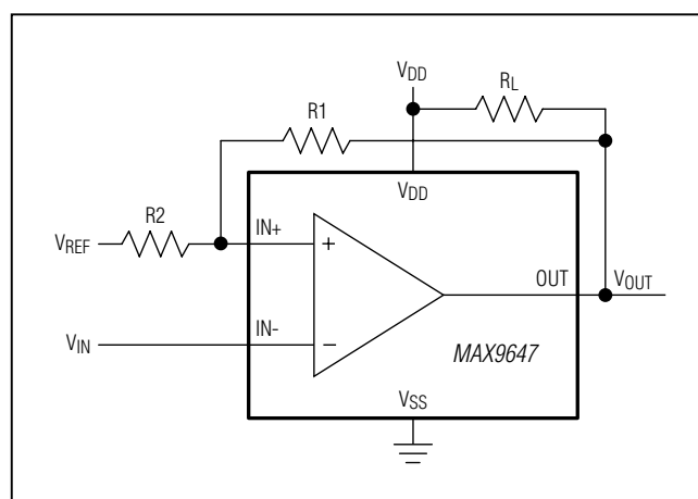
Figure 2. Adding Hysteresis with External Resistors
