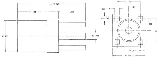
MMCX Straight PCB Mount Plug - Thru-Hole 908-22106
