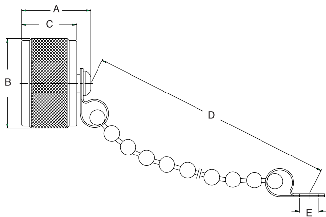
UHF Cap & Chain 83-1AC-RFX 83-1AC
