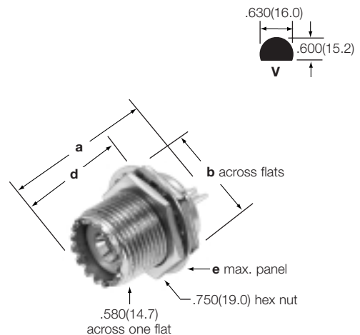
UHF Bulkhead Receptacle Rear Mount 83-878 83-878-1003 83-878-RFX
