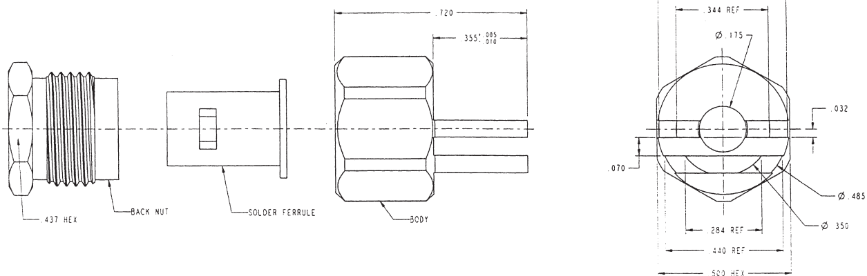
716-100 Edge Board Mount for 0.250 S/R Cable
