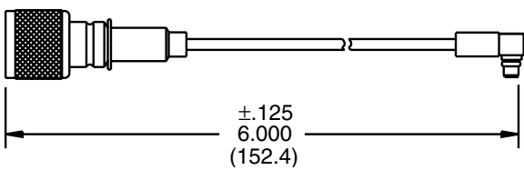
Right Angle MicroMate Plug to Straight Mini-UHF Plug 095-680-68000
