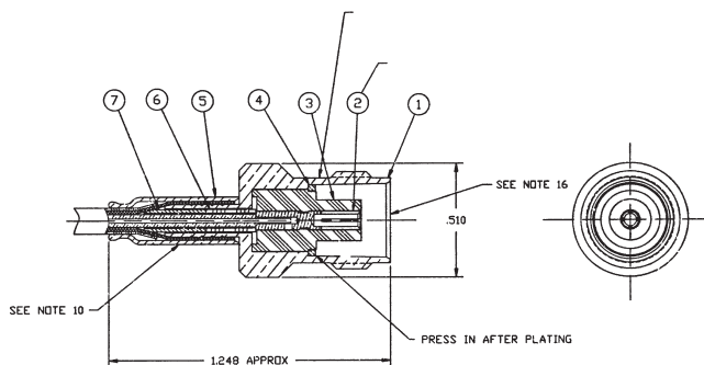
Cable Jack Assembly 79600 31-2317
