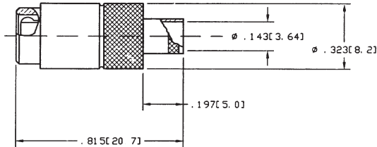
Straight Push-Pull Plugs Solder to Body 102-799-41 for .141 (3.6mm) SR RG 402 102-799-85 for .085 (2.2mm) SR RG 405
