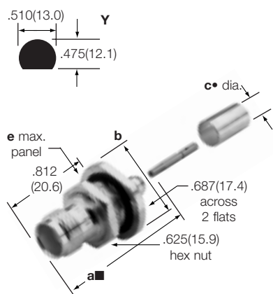
TNC Crimp Type Bulkhead Jack 31-2318 31-2264 31-2389 31-2264-RFX 31-2389-RFX
