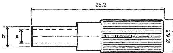
Straight Screw-On Plug 102-920-06 for RG-174, 188, 316
