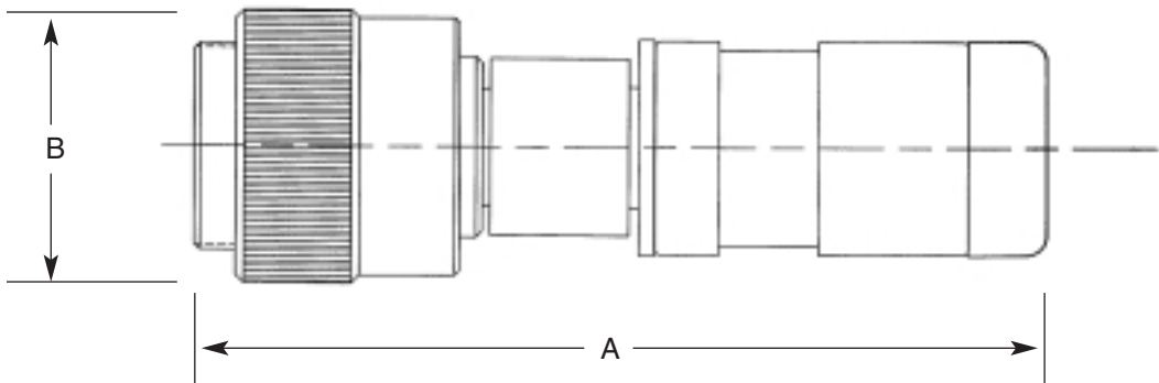
APC-7 for RG-214/U Cable 131-91032
