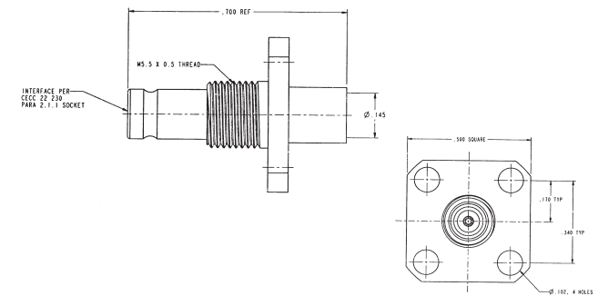
Straight 4-Hole Flange Jack 102-243-41 for SR .141
