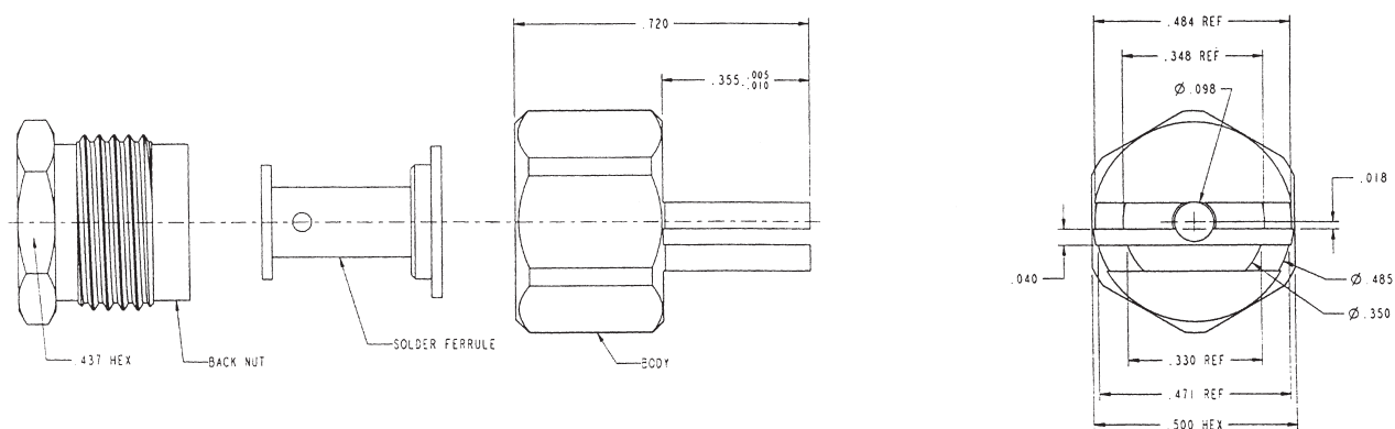
716-101 Edge Board Mount for 0.141 S/R Cable
