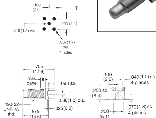
50Ω SMC PC Bulkhead Receptacle Male Contact/Post Terminal/Four Legs 903-421J-52P Gold Plated
