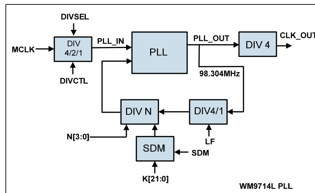
Figure 11 PLL Architecture
