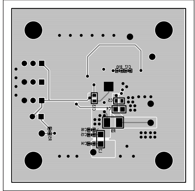
Figure 6. MAX20003 EV Kit PCB Layout—Solder Side
