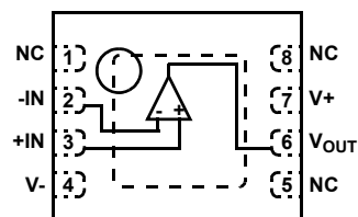
ISL28107 (8 LD TDFN) TOP VIEW
