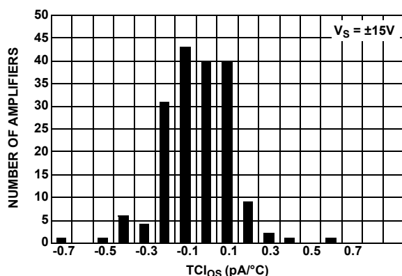
FIGURE 19. TC_{los} vs NUMBER OF AMPLIFIERS, V_S = \pm 15V
