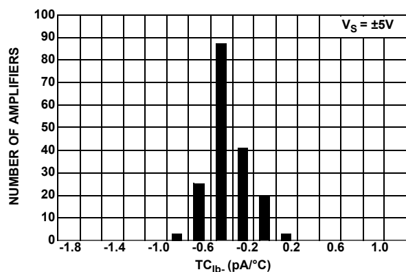
FIGURE 15. TC_{ibo} vs NUMBER OF AMPLIFIERS, V_S = \pm 5V
