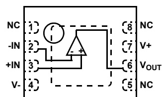
ISL28107 (8 LD TDFN) TOP VIEW
