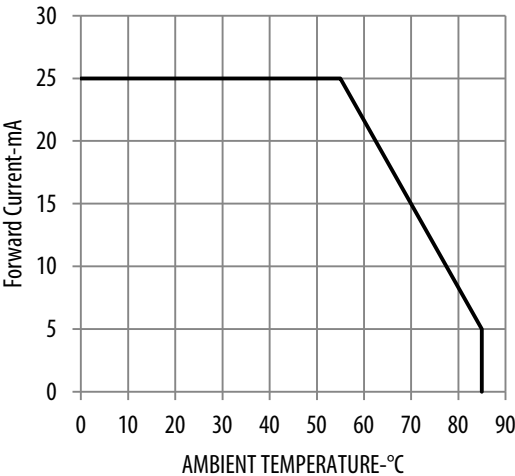
Figure 10: Derating Curve
