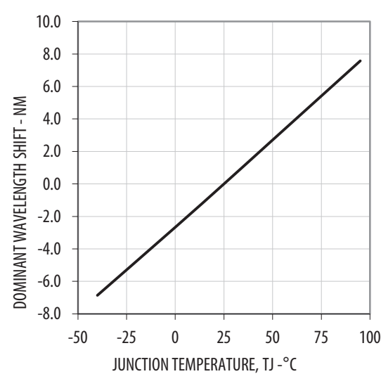
Figure 9: Wavelength Shift vs. Temperature
