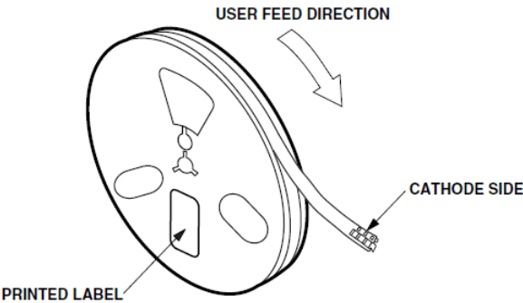
Figure 12: Reel Orientation
