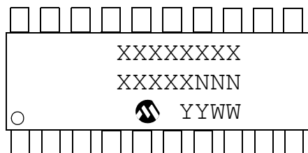
20-Lead TSSOP (All Devices)
