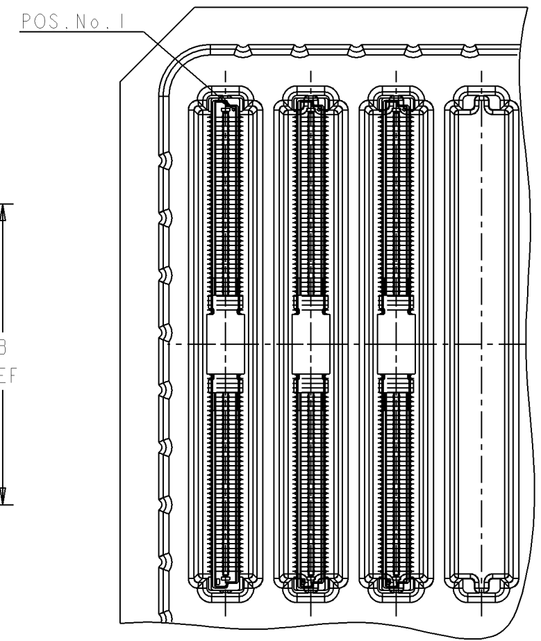
DETAIL "A" (1X EMPTY POCKET SHOWN FOR REF.)
