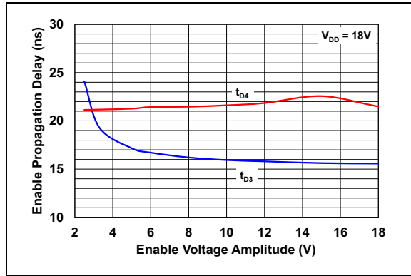
FIGURE 2-11: Enable Propagation Delay vs. Enable Voltage Amplitude.
