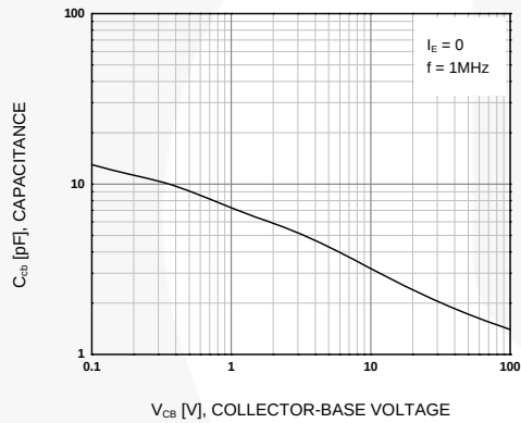
Figure 3. Collector-Base Capacitance
