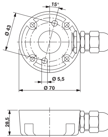
Dimensioned drawing
