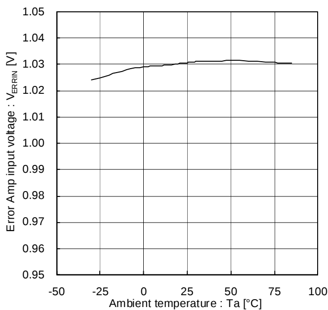
Figure 10. Error amplifier threshold voltage (Temperature dependency)
