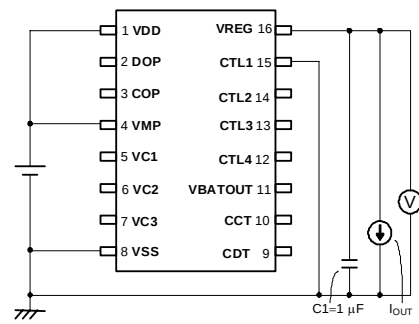
Test circuit 2
