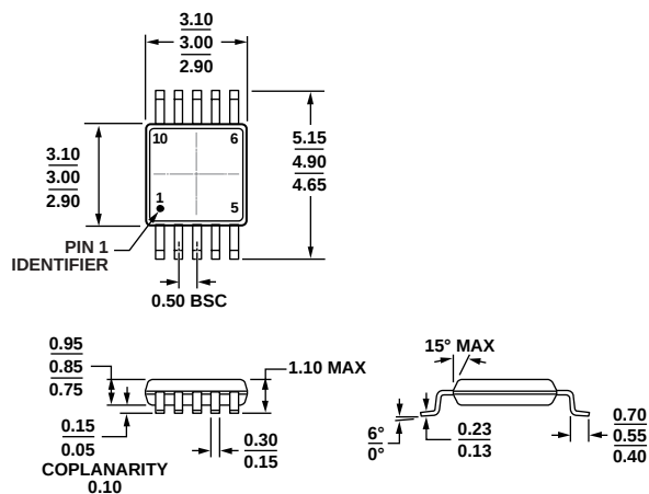
COMPLIANT TO JEDEC STANDARDS MO-187-BA Figure 57. 10-Lead Mini Small Outline Package [MSOP] (RM-10)
