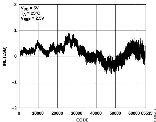
Figure 11. AD5683R/AD5683 INL
