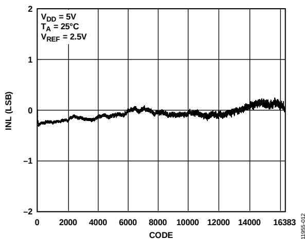
Figure 12. AD5682R INL
