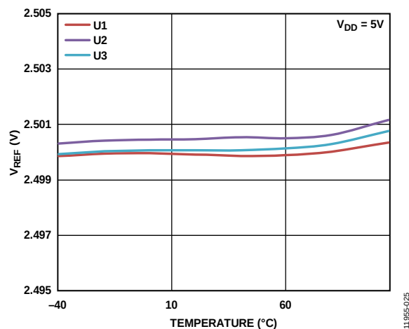
Figure 25. Internal Reference Voltage vs. Temperature (Grade B)
