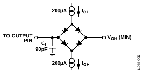
Figure 5. Load Circuit for Digital Output (SDO) Timing Specifications
