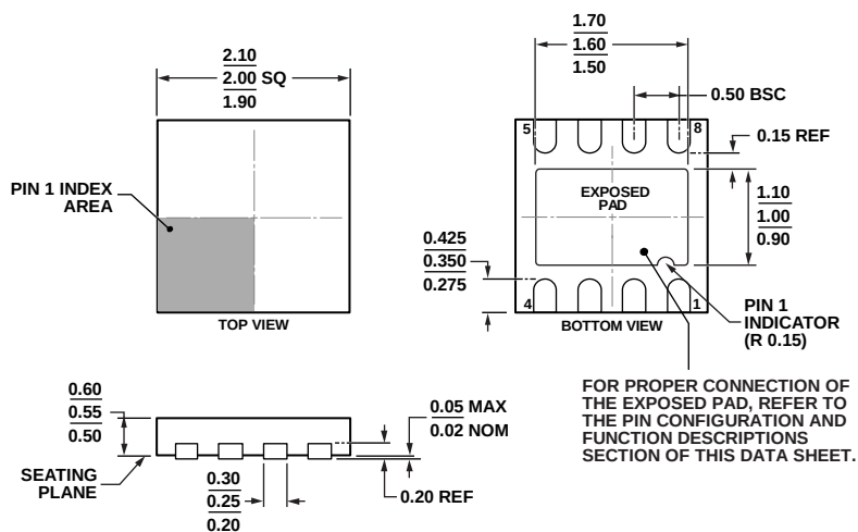
Figure 56. 8-Lead Lead Frame Chip Scale Package [LFCSP_UD] 2.00 mm x 2.00 mm Body, Ultrathin, Dual Lead (CP-8-10)
