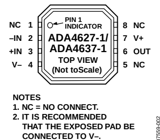
Figure 3. 8-Lead LFCSP_VD (CP-8-2)
