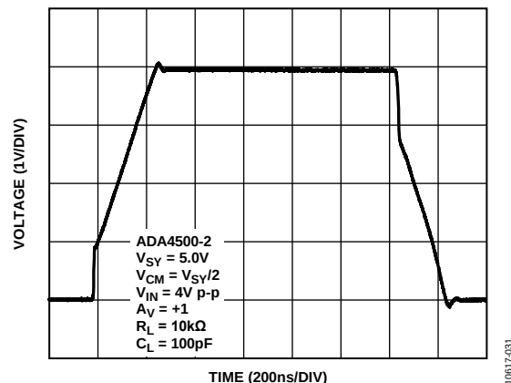
Figure 38. Large Signal Transient Response, V_{SV} = 5.0\text{ V}
