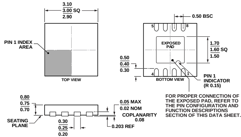
Figure 67. 8-Lead Lead Frame Chip Scale Package [LFCSP_WD] 3 mm × 3 mm Body, Very, Very Thin, Dual Lead (CP-8-12) Dimensions shown in millimeters
