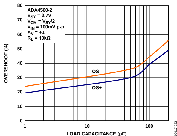
Figure 37. Small Signal Overshoot vs. Load Capacitance, V_{SV} = 2.7\text{ V}
