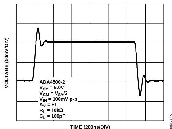
Figure 39. Small Signal Transient Response, V_{SV} = 5.0\text{ V}
