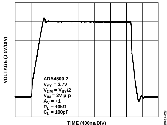
Figure 35. Large Signal Transient Response, V_{SV} = 2.7\text{ V}
