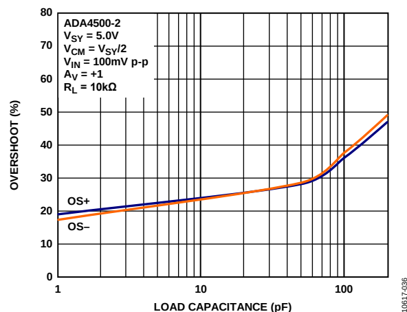
Figure 40. Small Signal Overshoot vs. Load Capacitance, V_{SV} = 5.0\text{ V}
