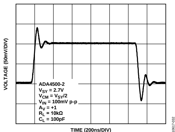
Figure 36. Small Signal Transient Response, V_{SV} = 2.7\text{ V}
