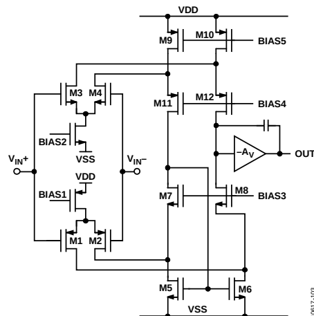
Figure 59. Typical PMOS-NMOS Rail-to-Rail Input Structure
