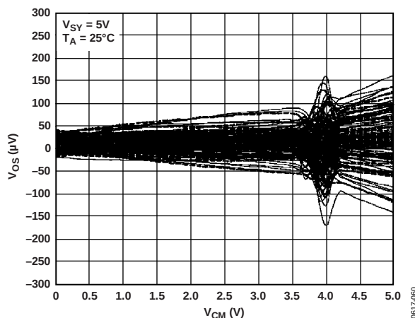
Figure 60. Typical Input Offset Voltage ( V_{OS} ) vs. Common-Mode Voltage ( V_{CM} ) Response in a Dual Differential Pair Input Stage Op Amp (Powered by a 5 V Supply; Results of Approximately 100 Units per Graph Are Displayed)
