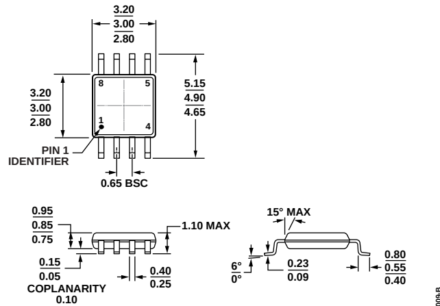
Figure 68. 8-Lead Mini Small Outline Package [MSOP] (RM-8)
