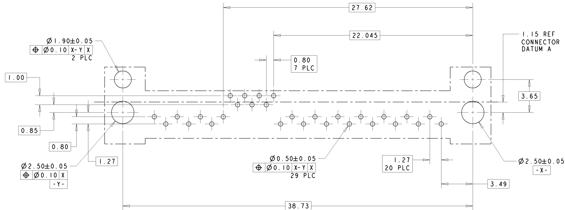
RECOMMENDED PCB LAYOUT SCALE 6:1
