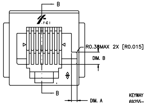
KEYED STYLE
