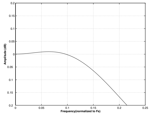
Figure 31. Quad Speed (fast) Passband Ripple
