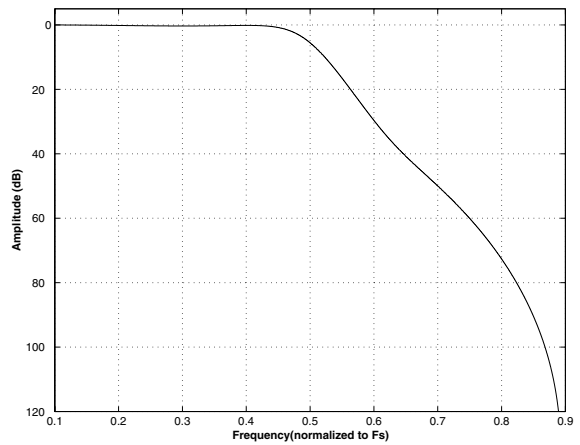
Figure 33. Quad Speed (slow) Transition Band
