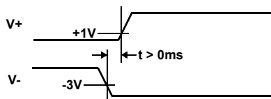
FIGURE 11. POWER SUPPLY SEQUENCING
