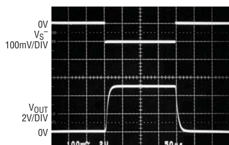
Step Response V_{\text{SENSE}} = 0\text{V to } 100\text{mV}, C_L = 1000\text{pF}, V_{\text{S}^+} = 0\text{V}
