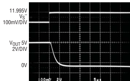
Step Response V_{\text{SENSE}} = 100\text{mV to } 5\text{mV}
