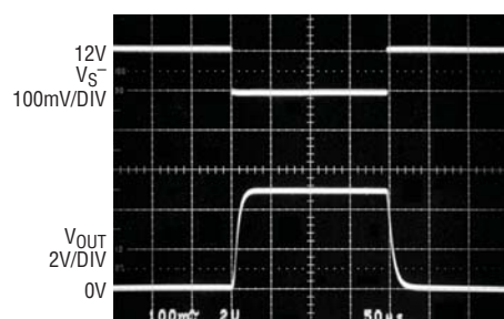
Step Response V_{\text{SENSE}} = 0\text{V to } 100\text{mV}, C_L = 1000\text{pF}, V_{\text{S}^+} = 12\text{V}
