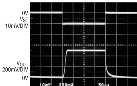
Step Response V_{\text{SENSE}} = 0\text{V to } 10\text{mV}, V_{\text{S}^+} = 0\text{V}
