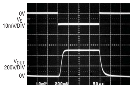
Step Response V_{\text{SENSE}} = 0\text{V to } 10\text{mV}, C_L = 1000\text{pF}, V_{\text{S}^+} = 0\text{V}
