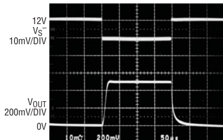
Step Response V_{\text{SENSE}} = 0\text{V to } 10\text{mV}, V_{\text{S}^+} = 12\text{V}
