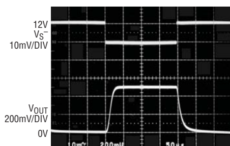
Step Response V_{\text{SENSE}} = 0\text{V to } 10\text{mV}, C_L = 1000\text{pF}, V_{\text{S}^+} = 12\text{V}
