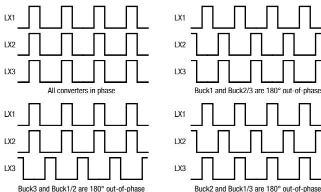
Figure 38. Out-of-Phase Operation
