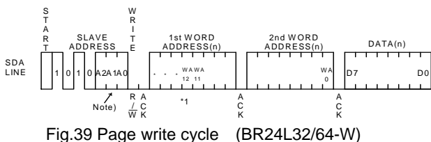
Fig.39 Page write cycle (BR24L32/64-W)
