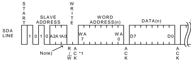
Fig.38 Page write cycle (BR24L01A/02/04/08/16-W)
