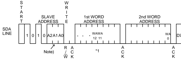
Fig.37 Byte write cycle (BR24L32/64-W)
