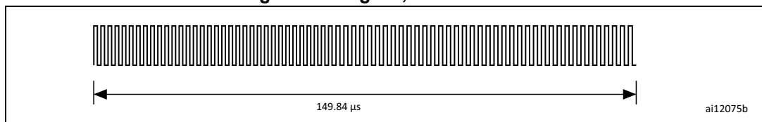
Figure 34. Logic 1, low data rate
