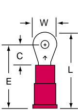
MVU18-2R/S Stud Size 2 Wire Range 22-18
