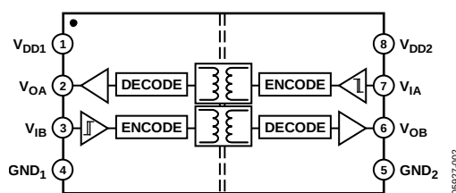
Figure 2. ADuM3201 Functional Block Diagram
