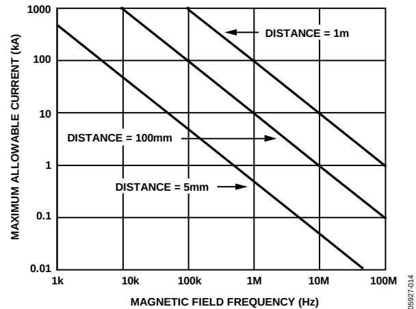
Figure 14. Maximum Allowable Current for Various Current-to- ADuM3200/ADuM3201 Spacings
