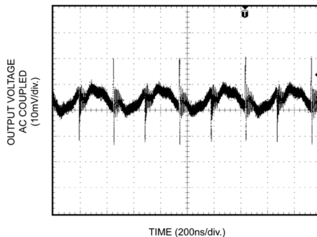
Output Ripple
