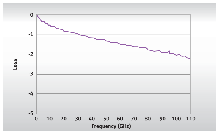
FIGURE 8: TYPICAL INSERTION LOSS 1
