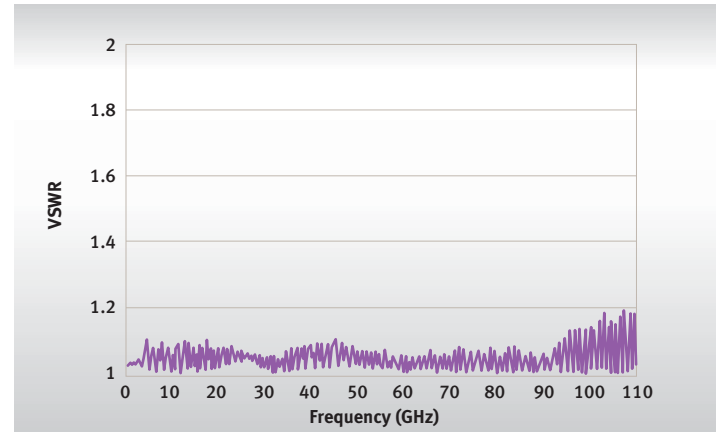
FIGURE 7: TYPICAL VSWR 1
