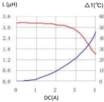
1. CDRR73NP-3R3MC
