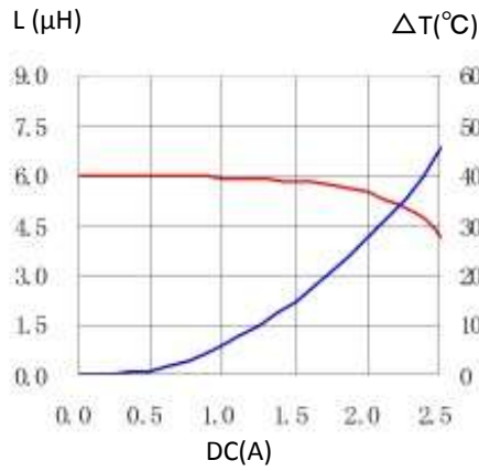
2. CDRR73NP-6R8MC
