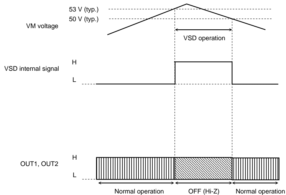
VSD operation
