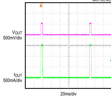
OUTPUT OVERLOAD PROTECTION OF MAX17502F, 5V OUTPUT, FIGURE 8 CIRCUIT
