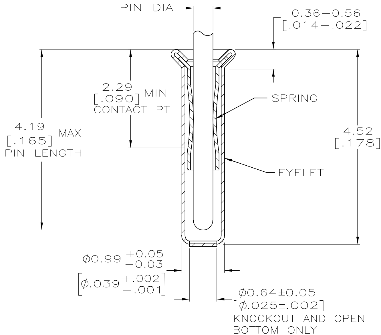
SECTION A—A
