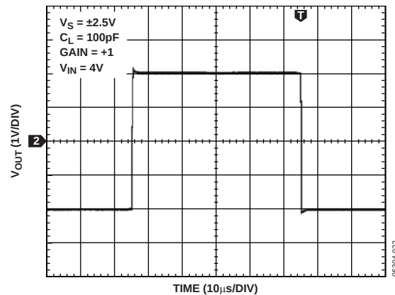
Figure 25. Large Signal Response
