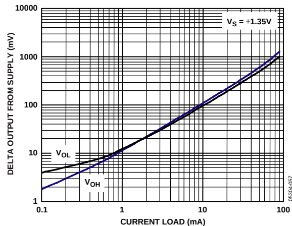
Figure 36. AD8656 Output Swing vs. Current Load
