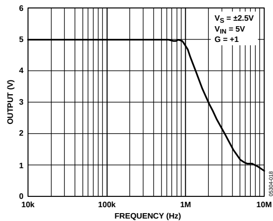
Figure 24. Maximum Output Swing vs. Frequency
