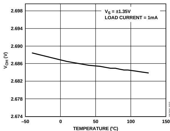
Figure 37. Output Voltage Swing High vs. Temperature
