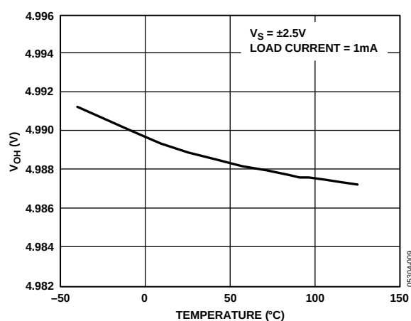
Figure 12. Output Voltage Swing High vs. Temperature
