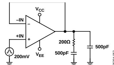
Figure 55. Snubber Network
